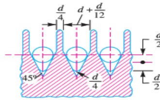
(b) Sheave (grooved pulley) for ropes.
