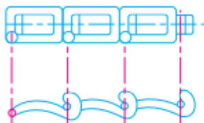
(a) Detachable or hook joint type chain.
