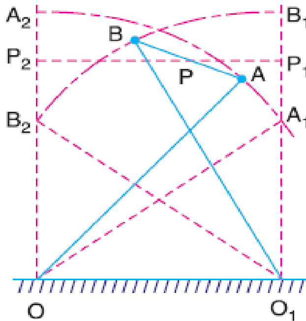
Fig. 2.8 Tchebicheff's mechanism
