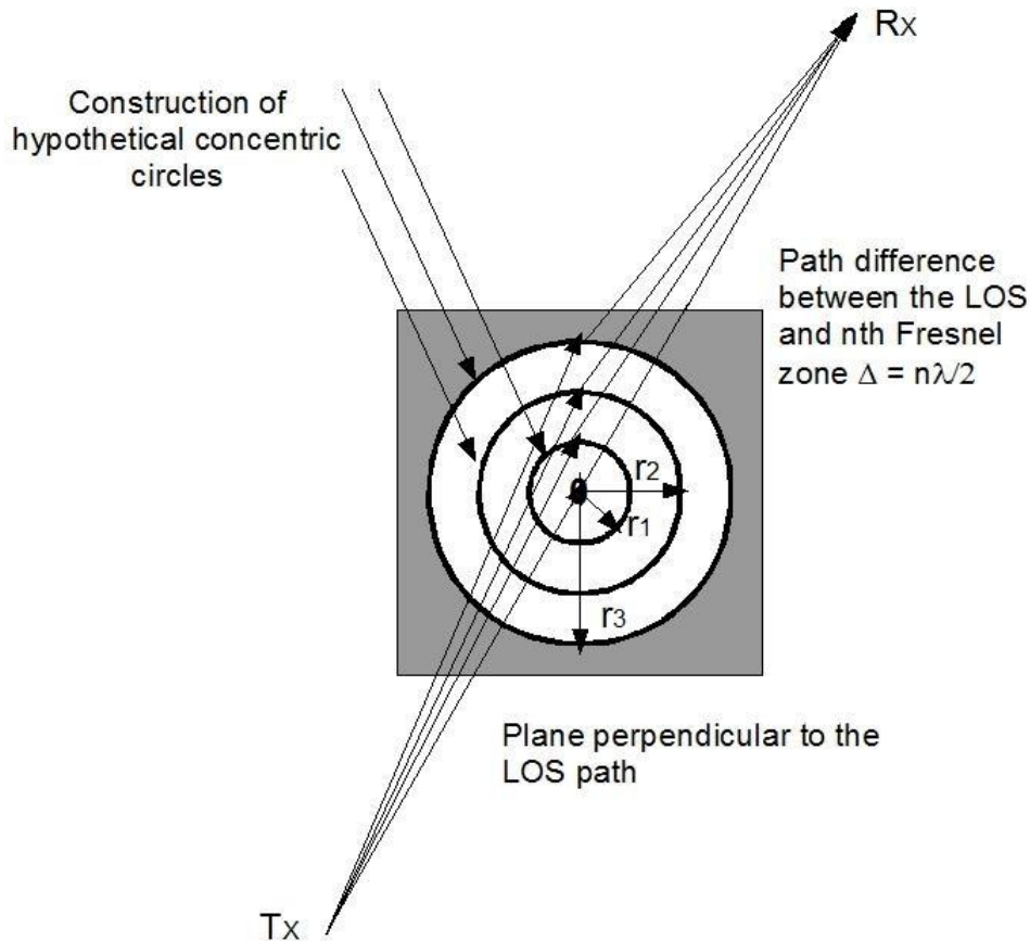
Figure 4.7: Fresnel
