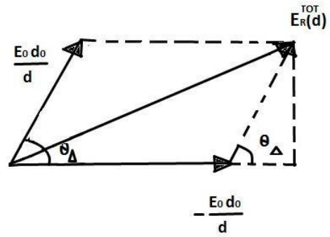
Figure 4.4: Equivalent phasor diagram of Figure 4.3.
